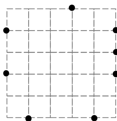
Isosceles Triangle
