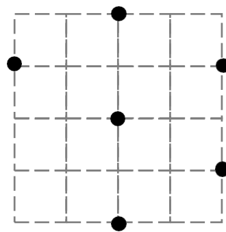
Right-angled Triangle
