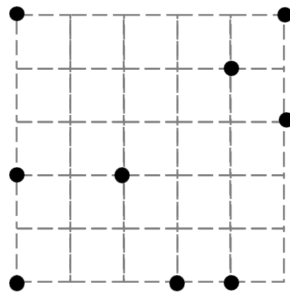
Parallelogram
