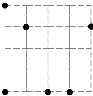
Isosceles Triangle
