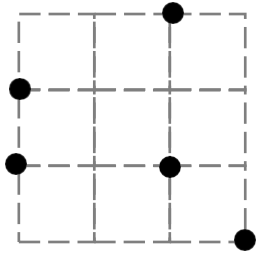
Right-angled Triangle
